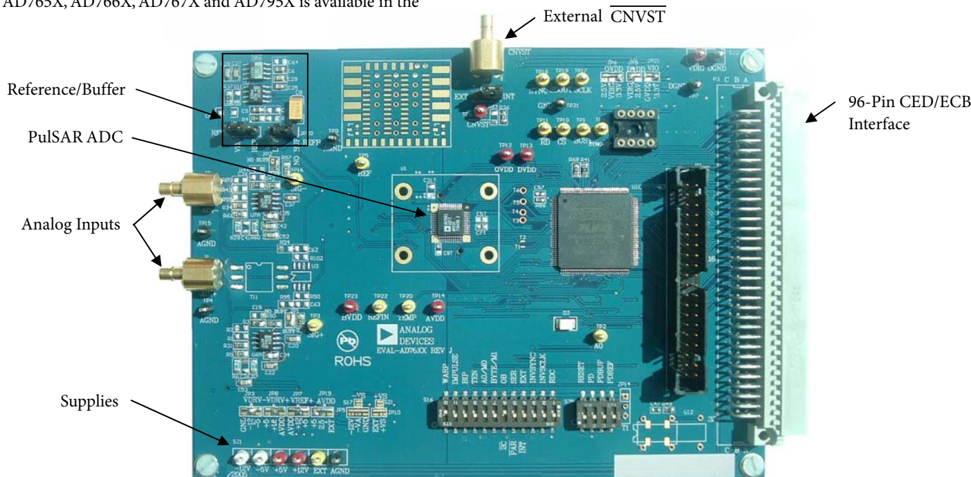
Figure 1. Evaluation Board
